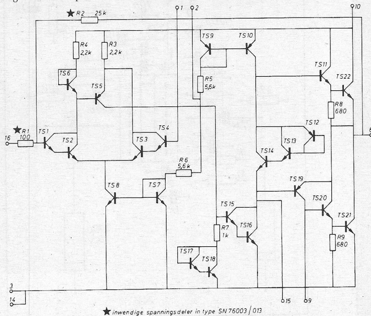
★ inwendige spanningdeler in type SN76003/013
